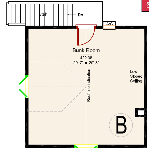
Pool House Upper Level
